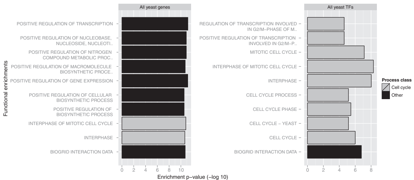
Figure 3. Comparison of standard, global background gene list (left plot) and customized list (right plot) in functional enrichment analysis of nine core cell cycle transcription factors in yeast. Top 10 enriched categories are shown vertically and log-scale P -values horizontally. R was used for visualization. The global analysis reveals general functional enrichments of transcriptional regulation (black bars), while focused analysis with the custom background of all yeast TFs shows specific cell cycle-related terms (grey bars).
